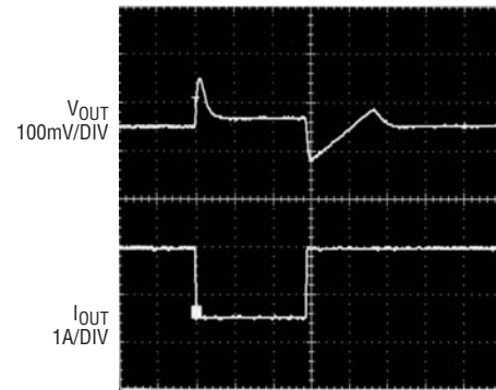
LT3015 Transient Response, C_{FF} = 10\text{nF}, C_{OUT} = 47\mu\text{F}
