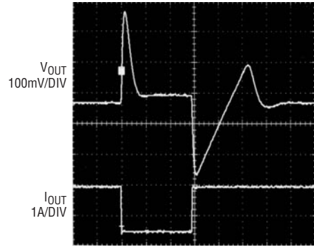
LT3015 Transient Response, C_{FF} = 0, C_{OUT} = 10\mu\text{F}
