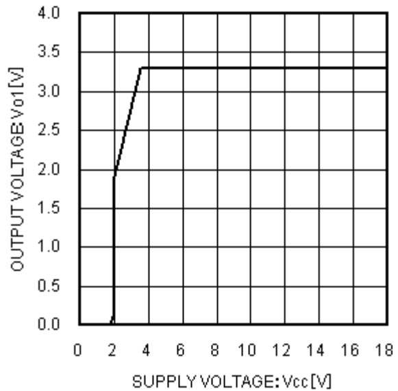
Fig.18 Input Stability (3.3 V output I_{o1}=600\text{ mA} )
