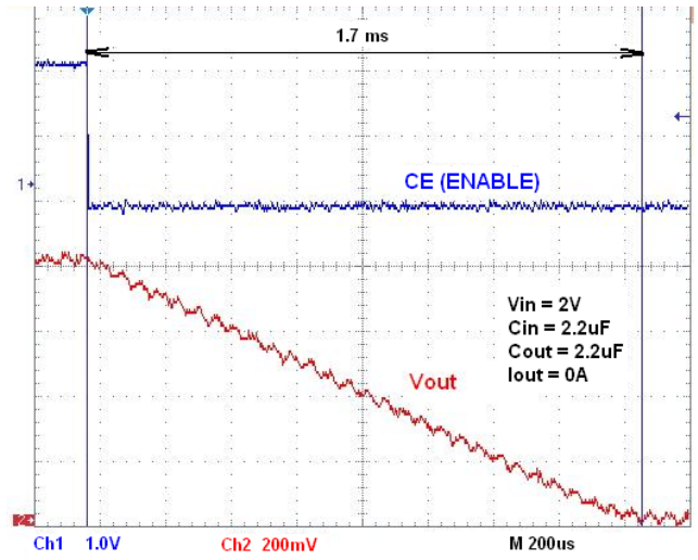
Figure 24. Turn Off Speed NCP693HMN08TCG
