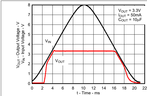
Figure 5-25. Power-Up, Power-Down (New Chip)
