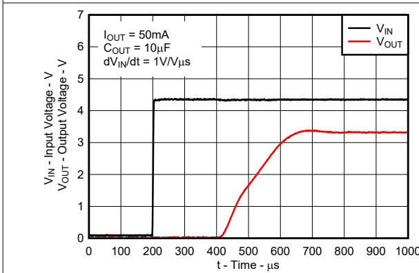
Figure 5-25. Power-Up, Power-Down (New Chip)
