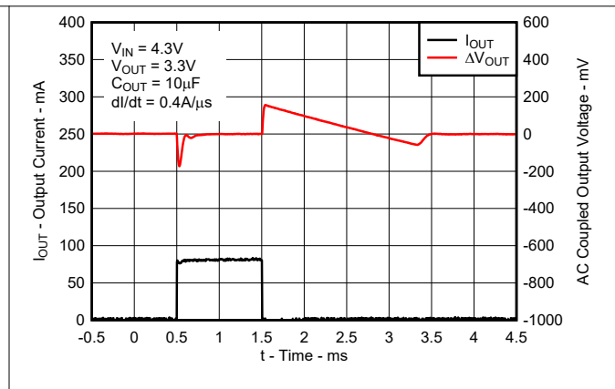
Figure 7-11. Load Transient Response (New Chip)
