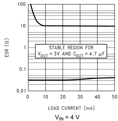
Figure 7-4. 3-V, 4.7-µF ESR Curves (Legacy chip)
