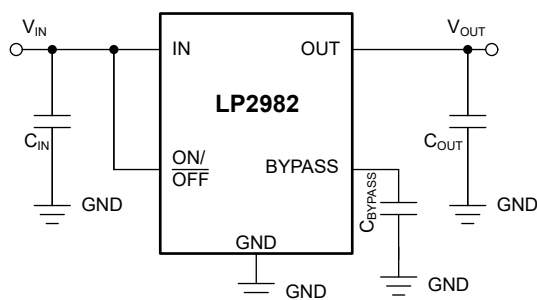
Simplified Schematic
