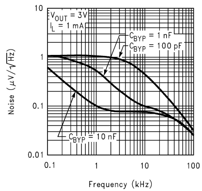
Figure 5-46. Output Noise Density (Legacy chip)
