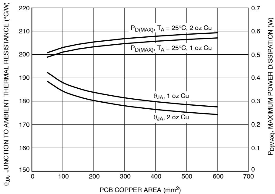
Figure 49. \theta_{JA} and P_D (MAX) vs. Copper Area – TSOP-5
