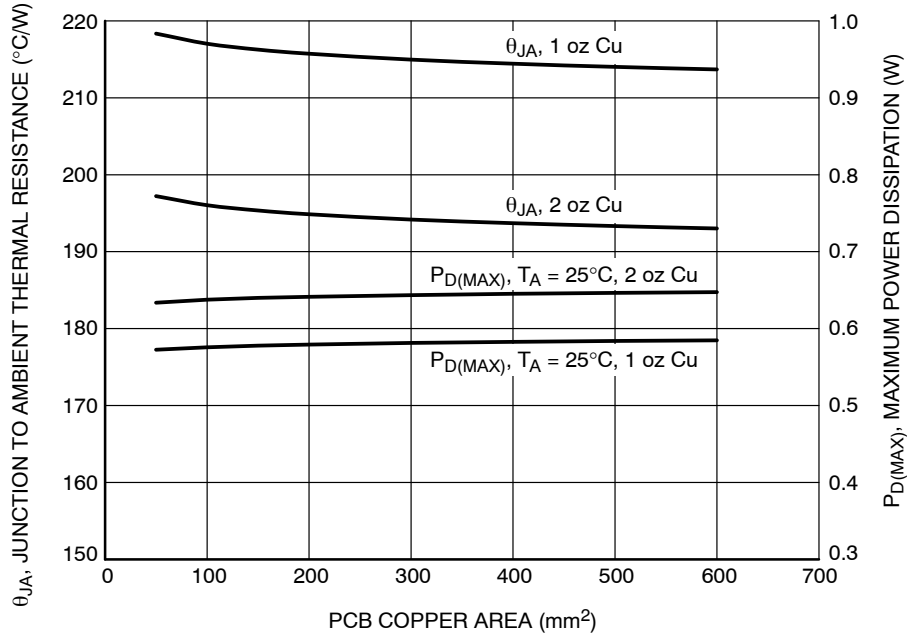
Figure 48. \theta_{JA} and P_D (MAX) vs. Copper Area – XDFN4
