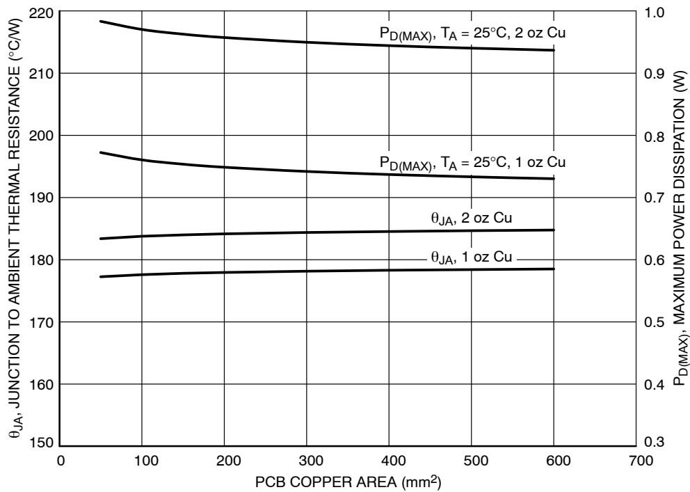
Figure 23. θ JA and P D(MAX) vs. Copper Area (XDFN4)
