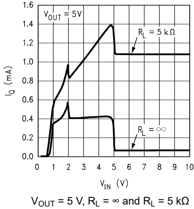
Figure 5-19. Input Current versus Input Voltage ( V_{IN} ) (Legacy Chip)
