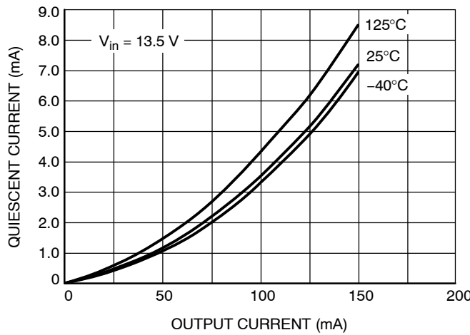
Figure 6. Current Consumption vs. Output Load, 5.0 V Version
