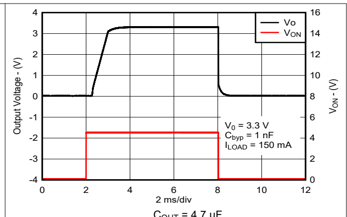
Figure 5-56. Turn-on Time for New Chip
