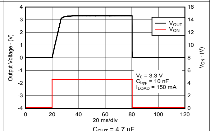
Figure 5-58. Turn-on Time for New Chip
