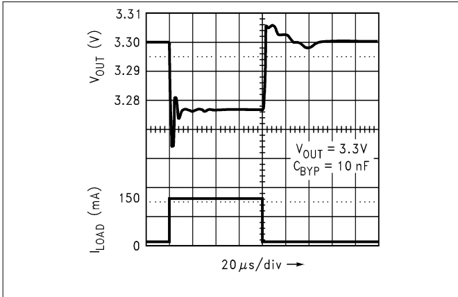
Figure 7-3. Load Transient Response for Legacy Chip
