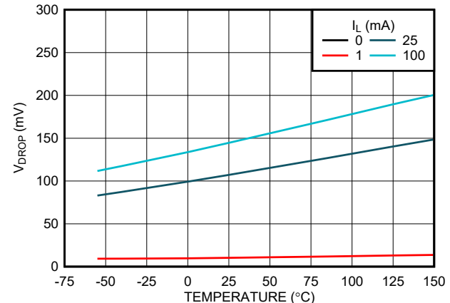
Dropout Voltage vs Temperature (New Chip)
