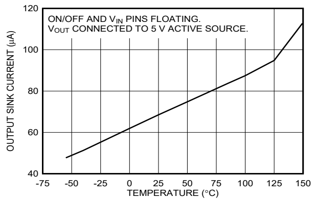
Figure 5-24. Output Reverse Leakage vs Temperature (New Chip)
