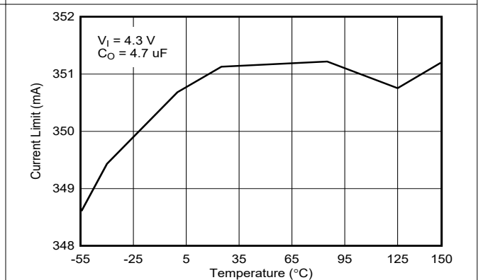
Figure 5-18. Instantaneous Short Circuit Current vs Temperature (New Chip)
