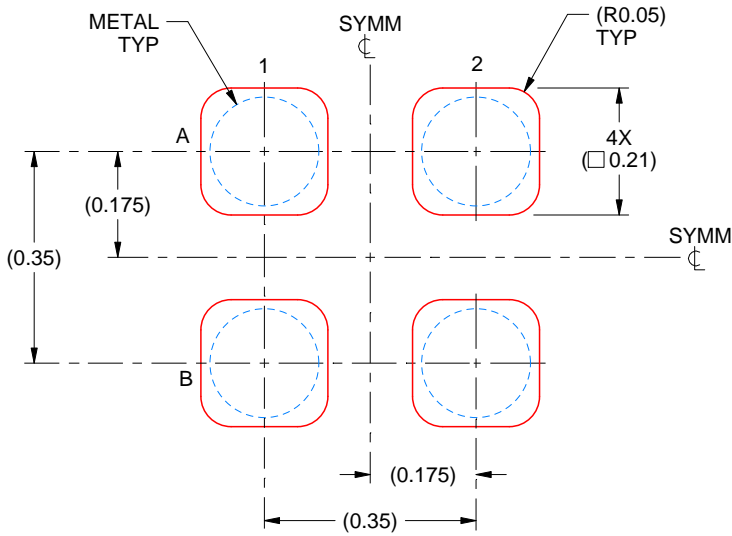
SOLDERPASTE EXAMPLE BASED ON 0.075 mm THICK STENCIL SCALE:80X
