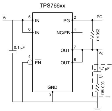
Typical Application Circuit
