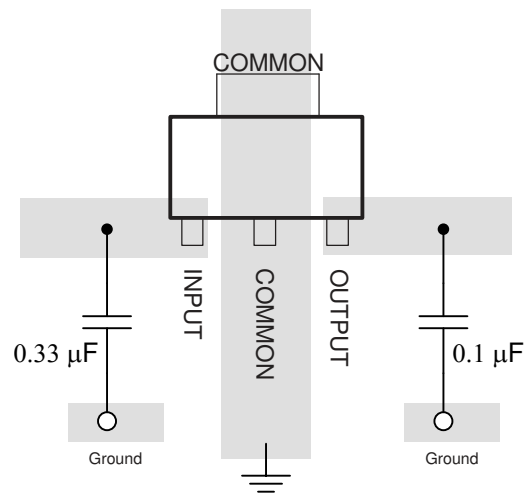
Figure 7-12. Layout Diagram
