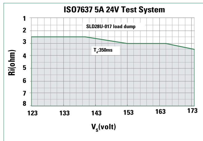
Figure 6 - SOA Chart
