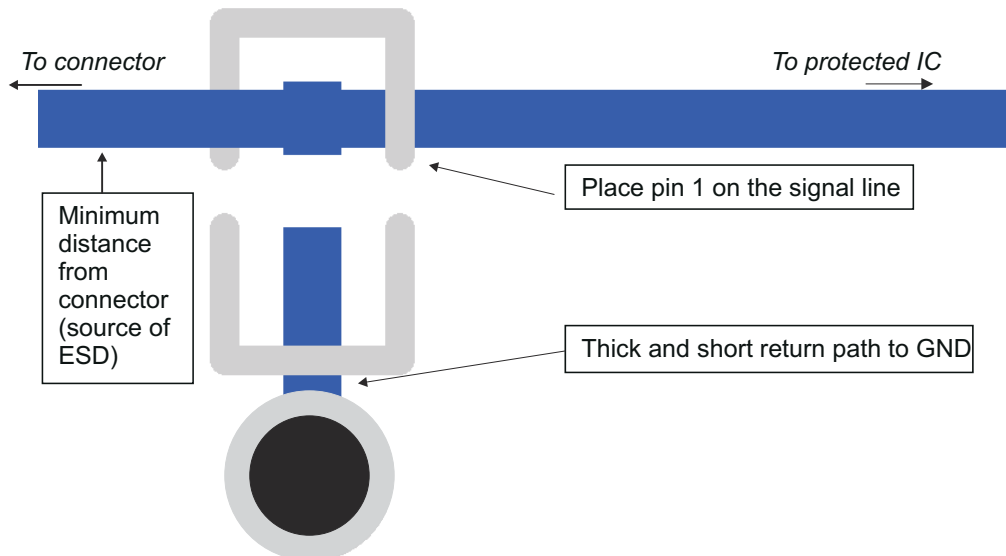
Figure 8-4. Layout Example
