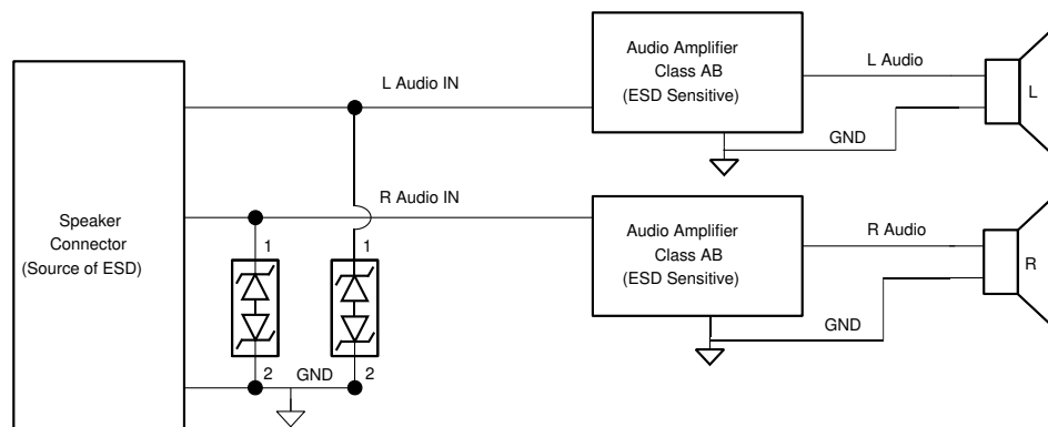
Figure 8-1. Typical Application Schematic
