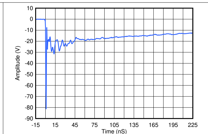
Figure 8-3. ESD Clamp Voltage –8-kV Contact ESD
