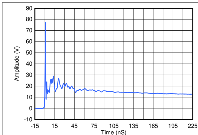
Figure 8-2. ESD Clamp Voltage 8-kV Contact ESD
