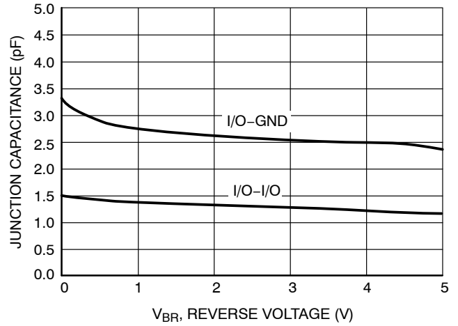
Figure 8. Junction Capacitance vs Reverse Voltage
