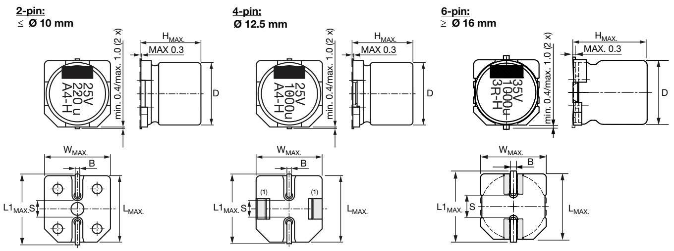
Fig. 2 - Dimensional outline
