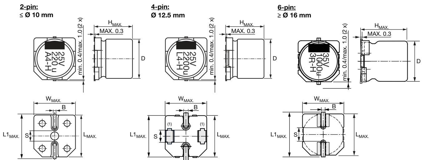
Fig. 2 - Dimensional outline
