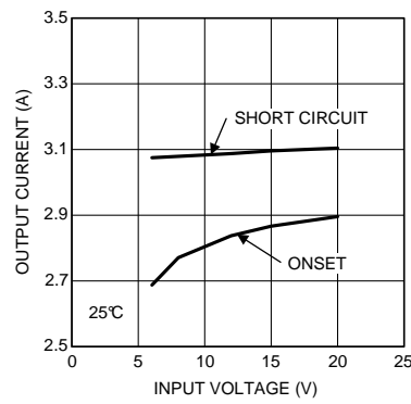
Figure 30. Current Limit 3.3 V OUT at 25°C
