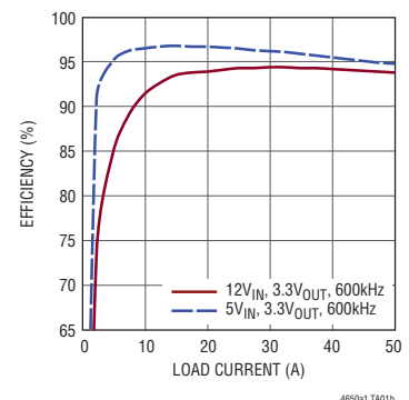
3.3V OUT Efficiency vs I OUT
