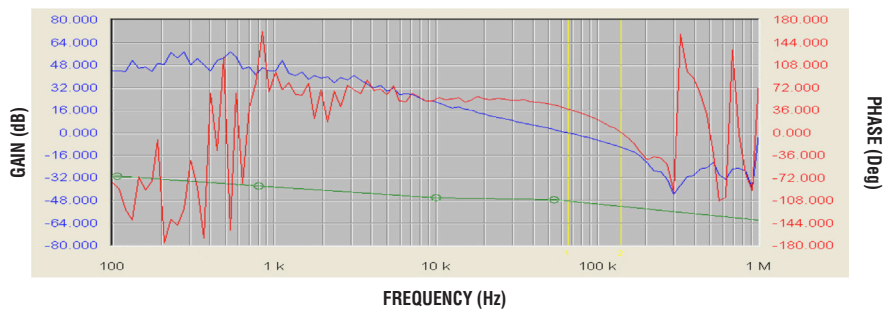
Figure 35. LTM4650A-1, 2-Phase, 1V at 50A Design with ±3% Transient Response
