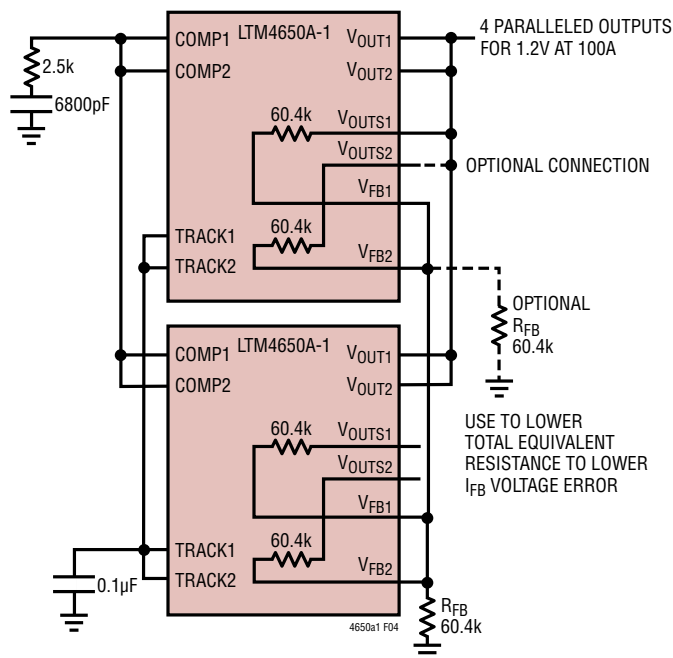
Figure 4. 4-Phase Parallel Configurations
