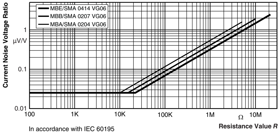
In accordance with IEC 60195 Current Noise Voltage Ratio
