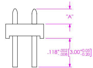
SHEAR VIEW FOR 05 & 06 LEAD STYLE
