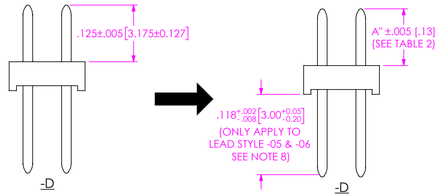
IN-PROCESS 2 (FOR -04 & -05 LEAD STYLE ONLY)
