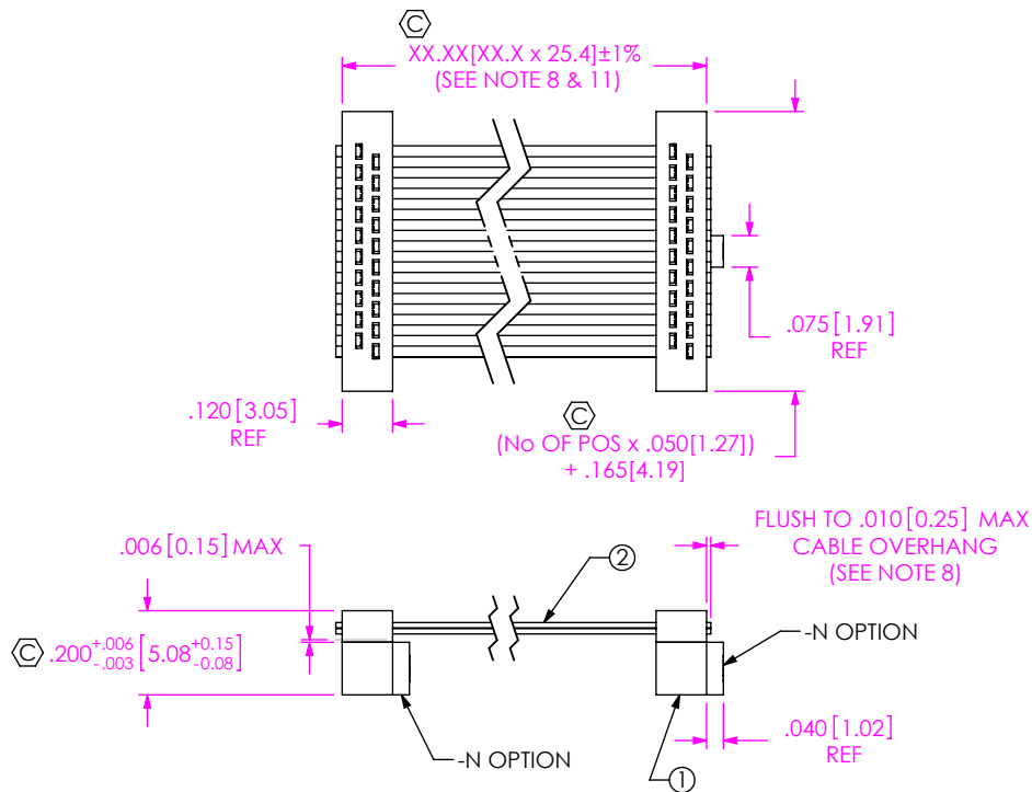
FIG 1 (FFSD-10-D-XX.XX-01-X-N SHOWN)
