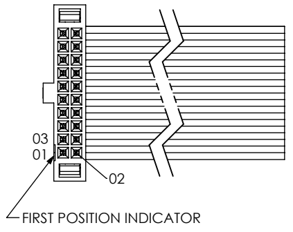
(FFSD-10-S-XX.XX-01-X-N-RN1 SHOWN) (SAME AS FIG 2, DIFFERENT AS SHOWN)
