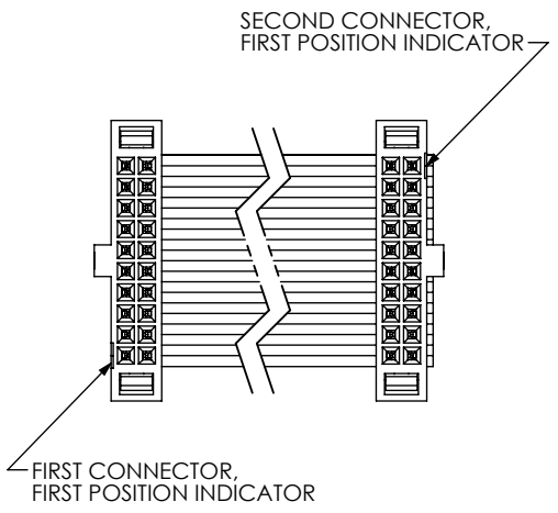
(FFSD-10-D-XX.XX-01-X-N-RN1 SHOWN) (SAME AS FIG 1, DIFFERENT AS SHOWN)
