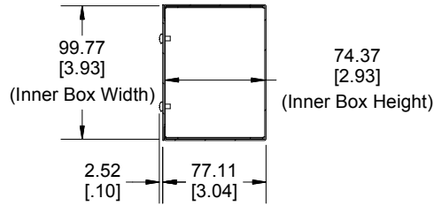
SECTION A-A End View of Assembly
